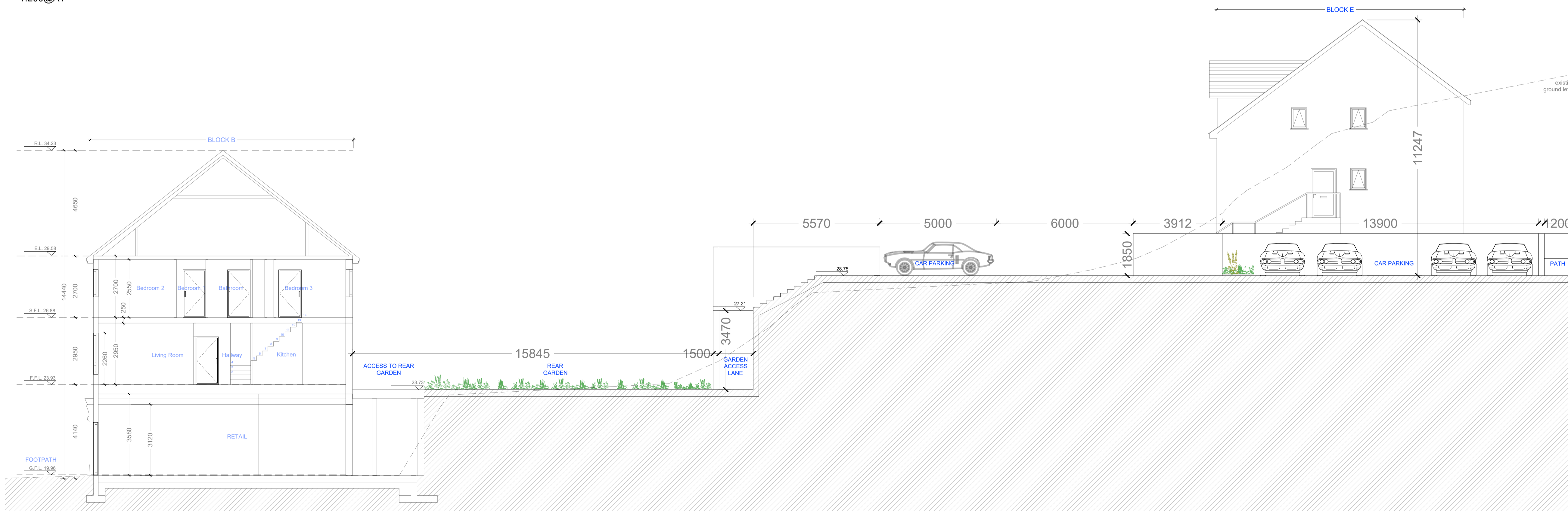
SITE SECTION 1 (SS-1) 1:100@A1
